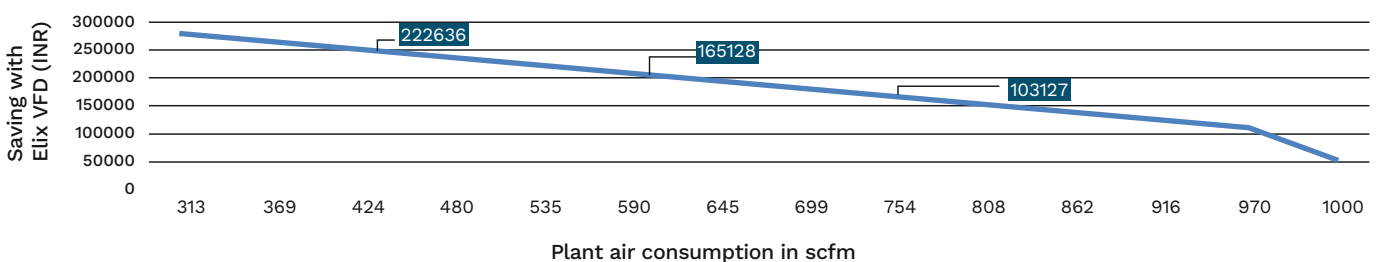
Pontential Saving (INR) per year with 1000cfm Elix VFD dryer under varying load condition
