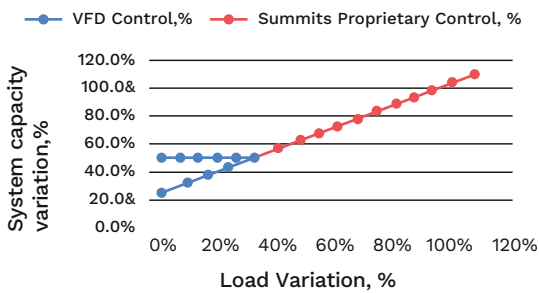
Elix VFD Control Scheme
